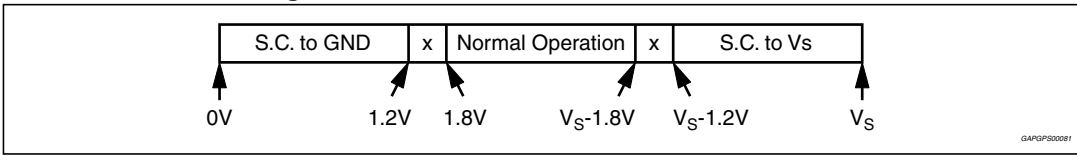
Figure 26. Short circuit detection thresholds
